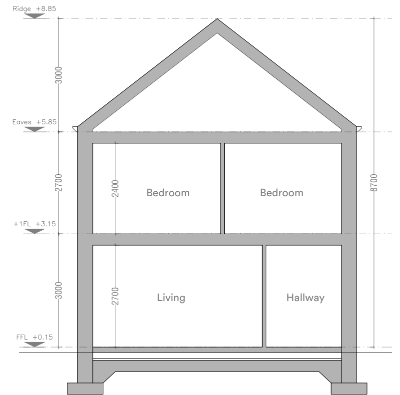
House Type M1 Detached Section A.A
