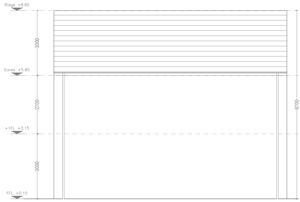
House Type M1 Detached Side Elevation
